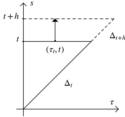
Fig. 2.3. Steepest ascent with Dini derivatives
